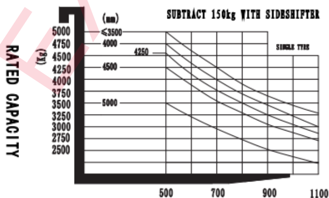
RATED CAPACITIES AND LOAD CENTERS GRAPH
